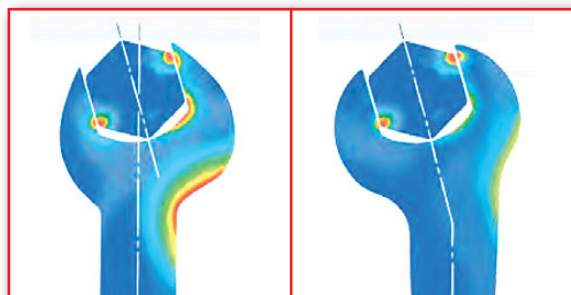
Load zones for conventional open ended spanner.
